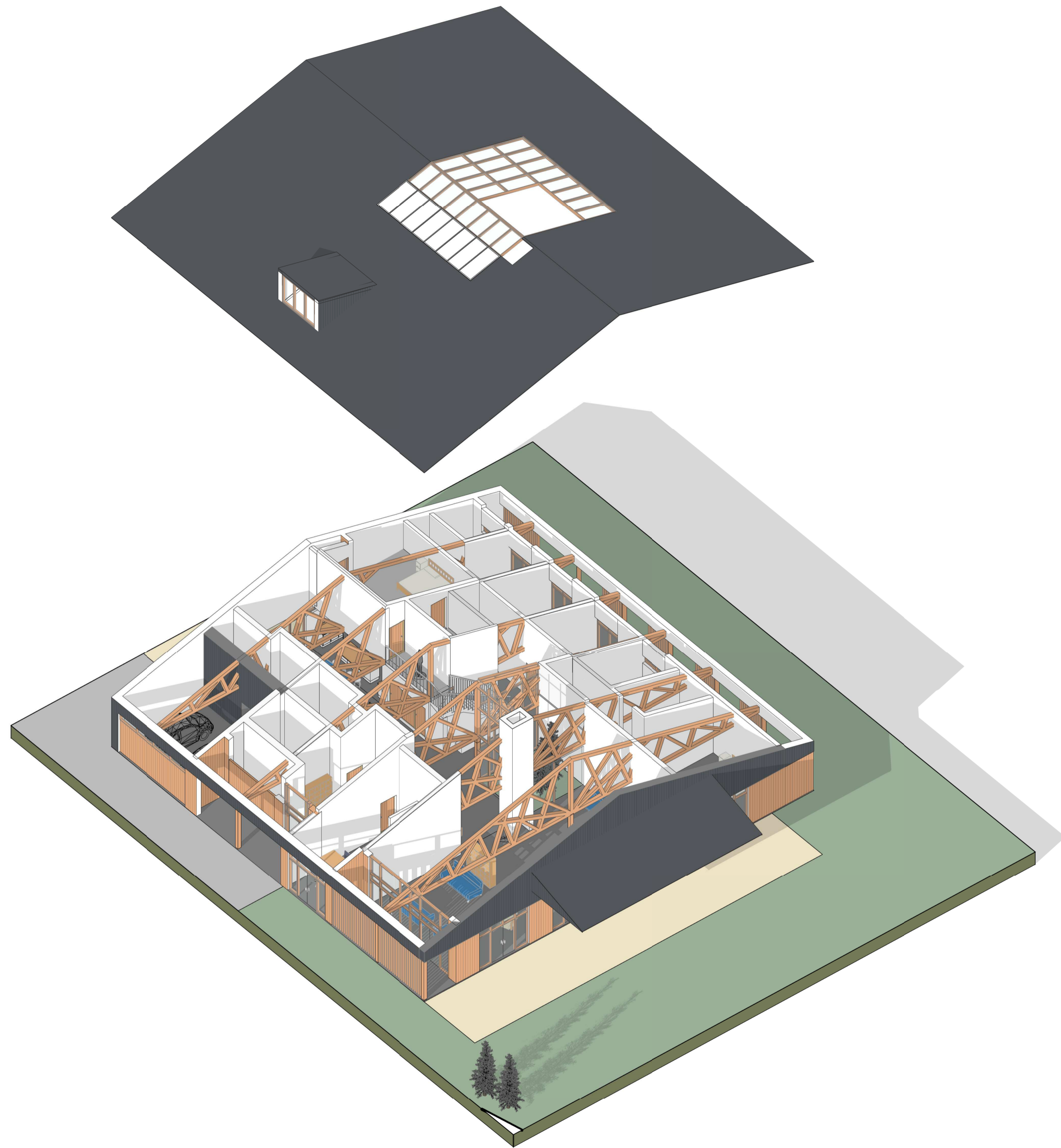
3D view from South East
